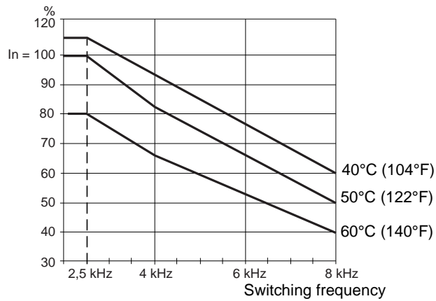
ATV71HD55M3X, HD75M3X
