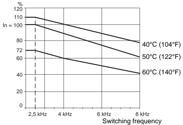
ATV71HC31N4
