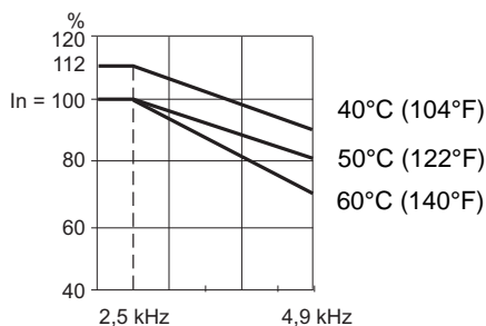
ATV71HC25Y
