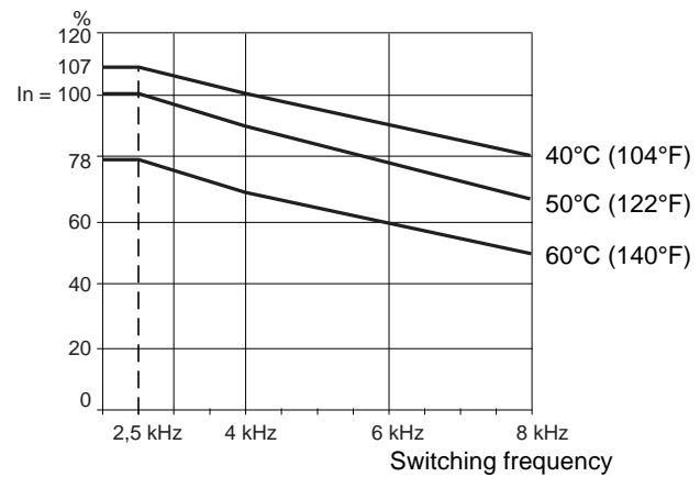
ATV71HC13N4
